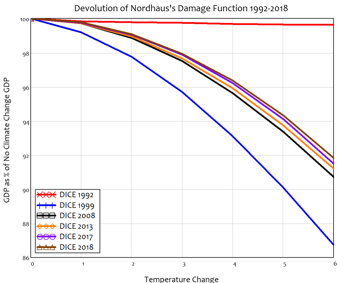
Figure 4: How low can you go? Nordhaus's downward revisions to his damage function
