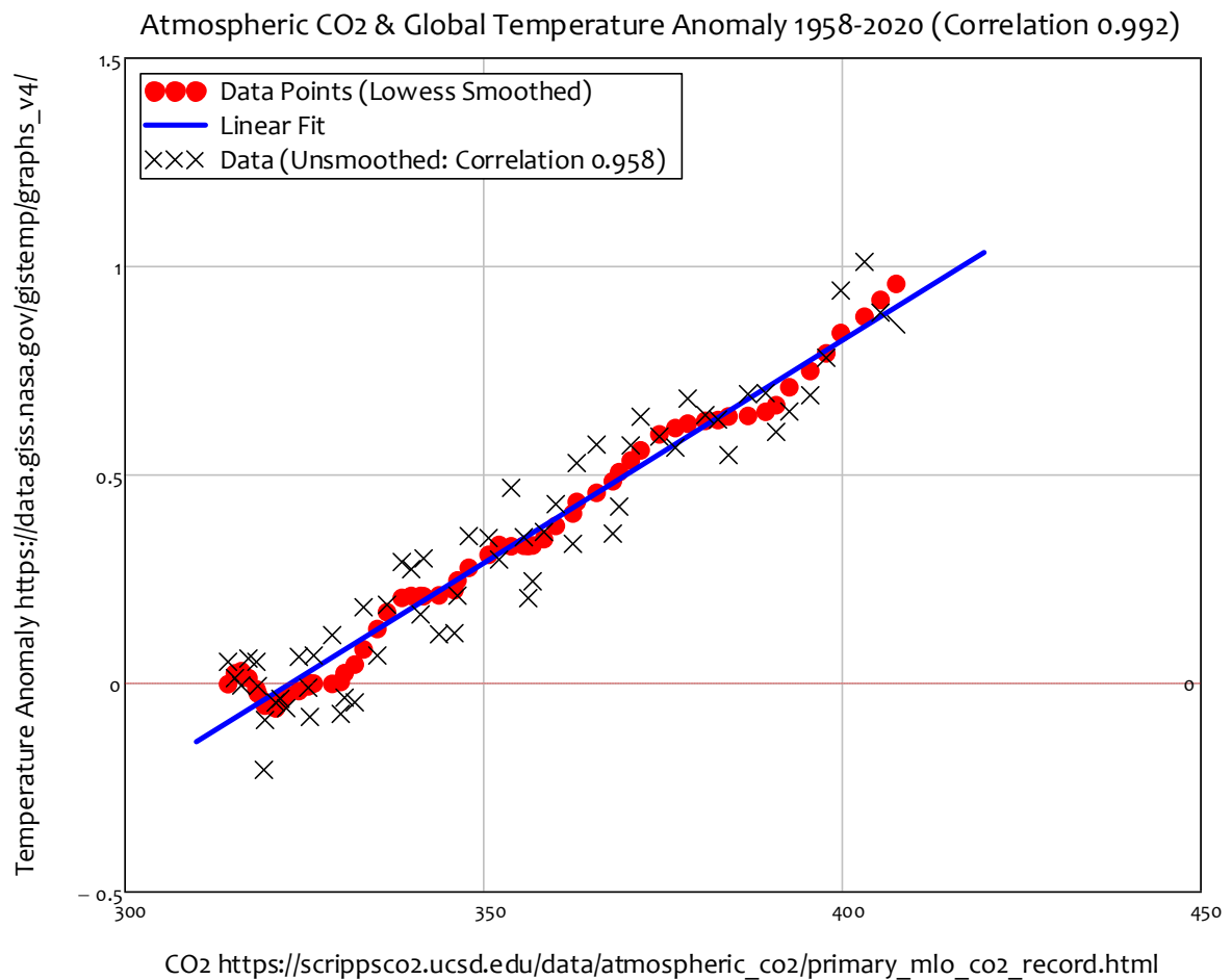
Figure 7: CO2 determines Global Warming
