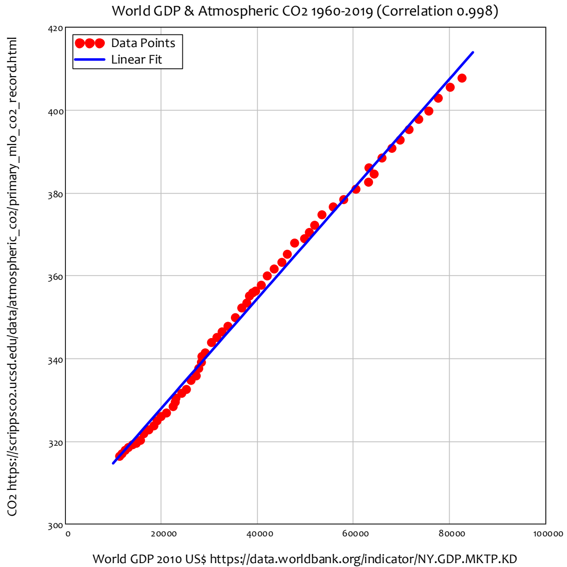
Figure 6: Without significant de-carbonization, GDP determines CO2
